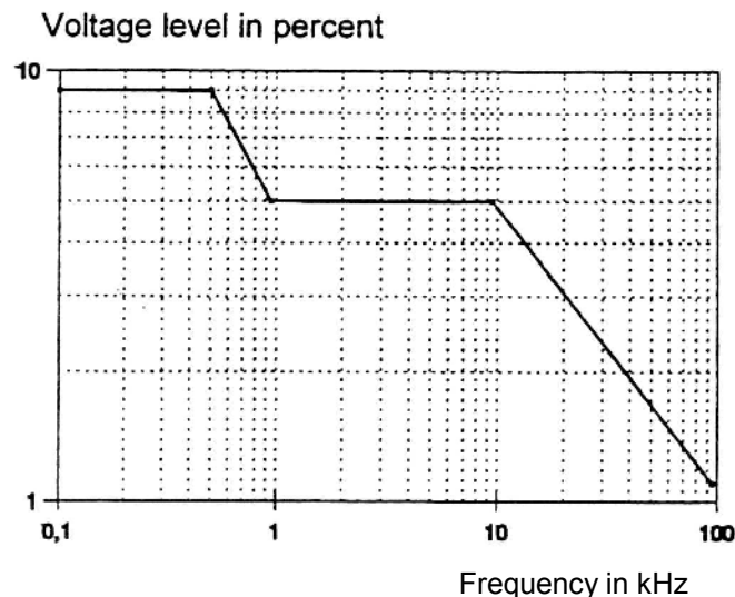
Figure 2 — Voltage levels of signal frequencies in percent of U_n used in public LV distribution systems
